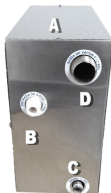
Vista Frontal
